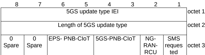
Figure 9.11.3.9A.1: 5GS update type information element
