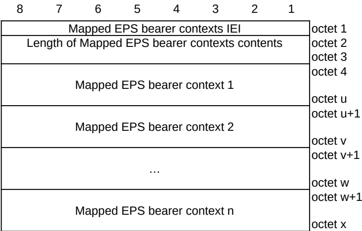
Figure 9.11.4.8.1: Mapped EPS bearer contexts
