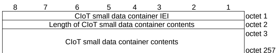
Figure 9.11.3.18B.1: Clot small data container information element
