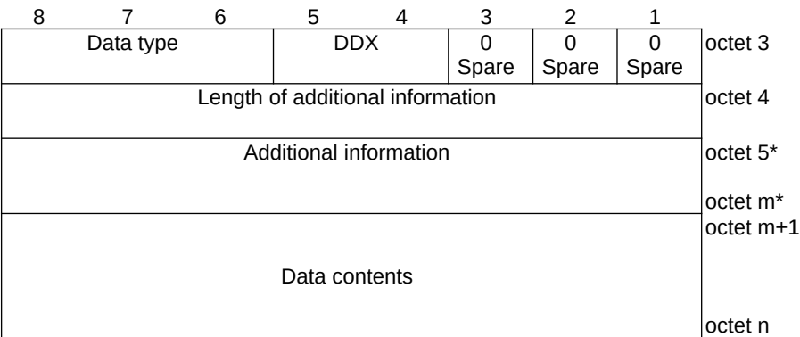
Figure 9.11.3.18B.3: ClIoT small data container contents for Data type "Location services message container"
