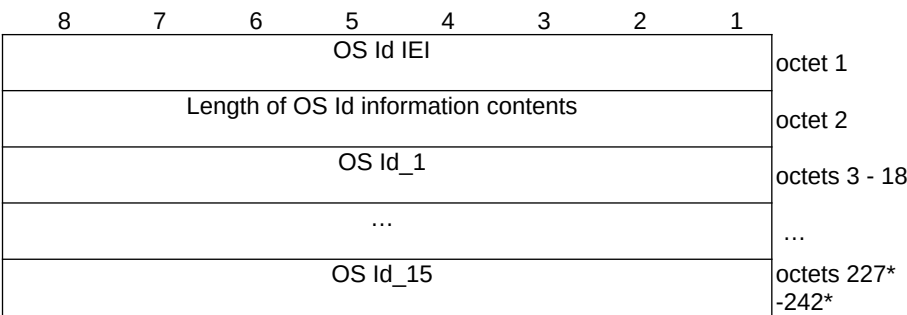
Figure D.6.6.1: UE OS Id information element
