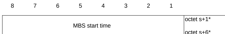
Figure 9.11.4.31.8: MBS timers for MBS timer indication = "MBS start time"
