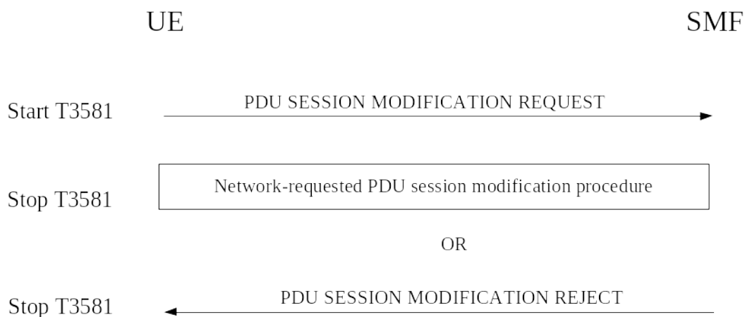
Figure 6.4.2.2.1: UE-requested PDU session modification procedure
