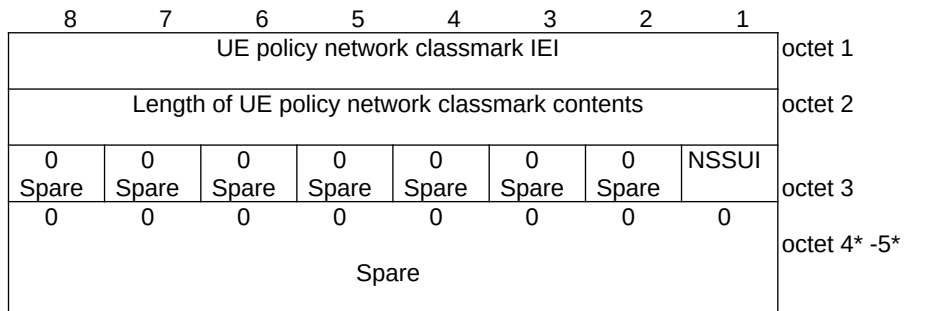
Figure D.6.7.1: UE policy network classmark information element
