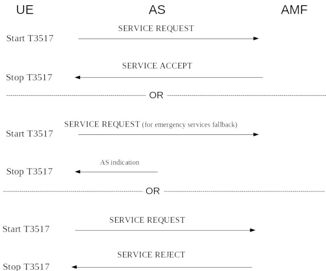
Figure 5.6.1.1.1: Service Request procedure (Part 1)
