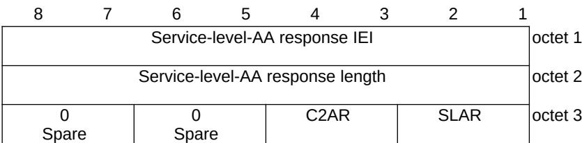
Figure 9.11.2.14.1: Service-level-AA response information element
