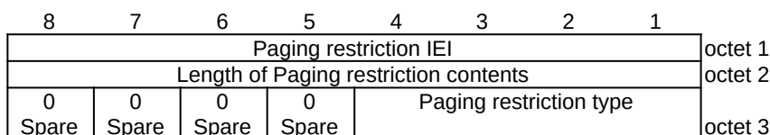
Figure 9.11.3.77.1: Paging restriction information element for Paging restriction type = "All paging is restricted" and for Paging restriction type = "All paging is restricted except voice"
