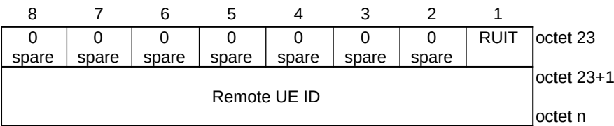
Figure 9.11.3.89.2: Remote UE identity
