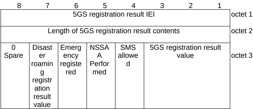
Figure 9.11.3.6.1: 5GS registration result information element
