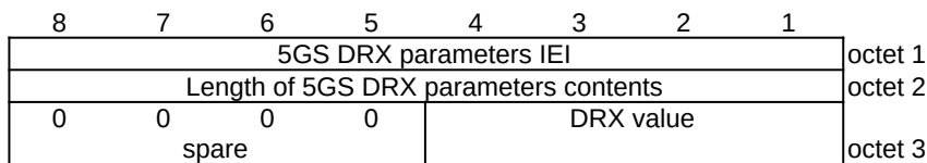
Figure 9.11.3.2A.1: 5GS DRX parameters information element
