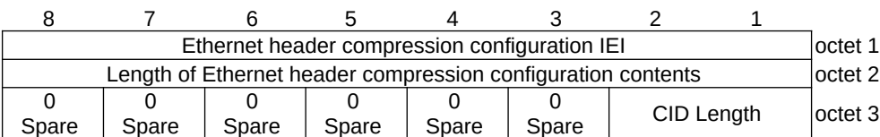
Figure 9.11.4.28.1: Ethernet header compression configuration information element
