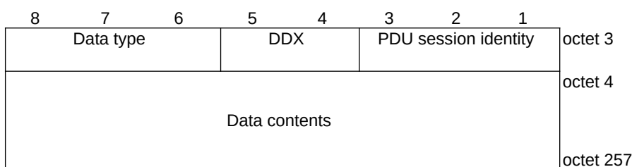
Figure 9.11.3.18B.2: Clot small data container contents for Data type "Control plane user data"
