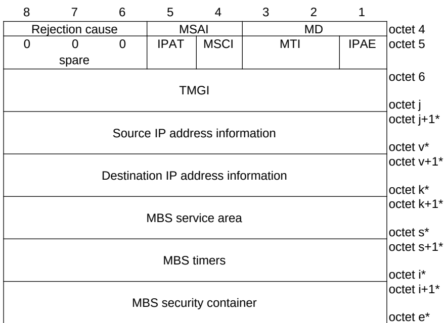
Figure 9.11.4.31.2: Received MBS information
