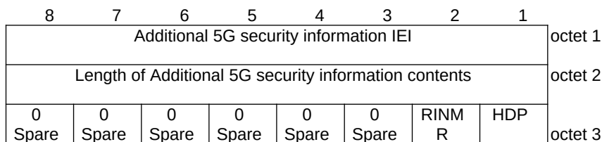
Figure 9.11.3.12.1: Additional 5G security information information element
