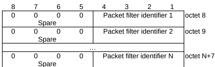
Figure 9.11.4.13.3: Packet filter list when the rule operation is "modify existing QoS rule and delete packet filters" (z=N+7)
