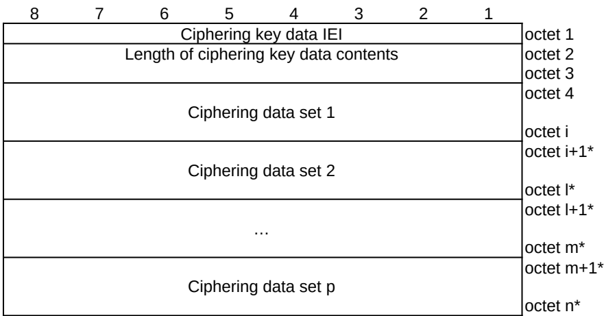
Figure 9.11.3.18C.1: Ciphering key data information element
