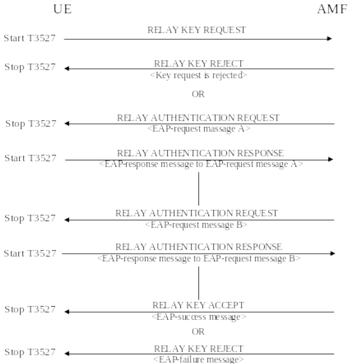
Figure 5.5.4.1.1: Authentication and key agreement procedure for 5G ProSe UE-to-network relay
