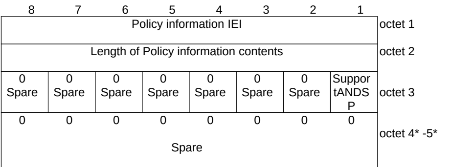
Figure D.6.5.1: UE policy classmark information element
