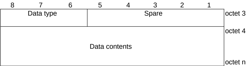
Figure 9.11.3.18B.4: ClIoT small data container contents for Data type "SMS"
