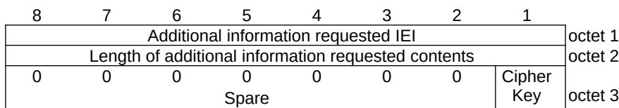
Figure 9.11.3.12A.1: Additional information requested information element
