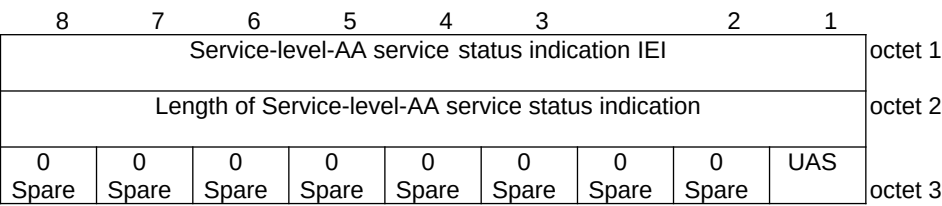
Figure 9.11.2.18.1: Service-level-AA-service-status indication information element
